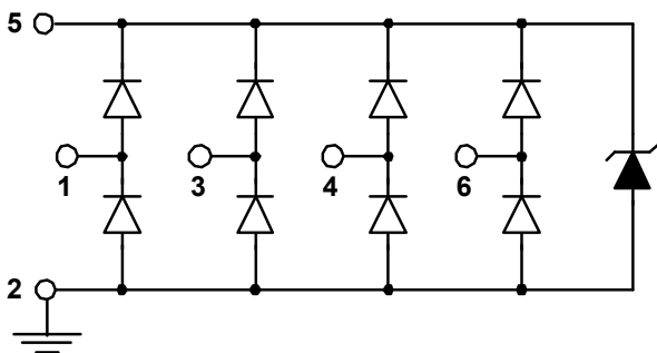
Circuit Diagram
